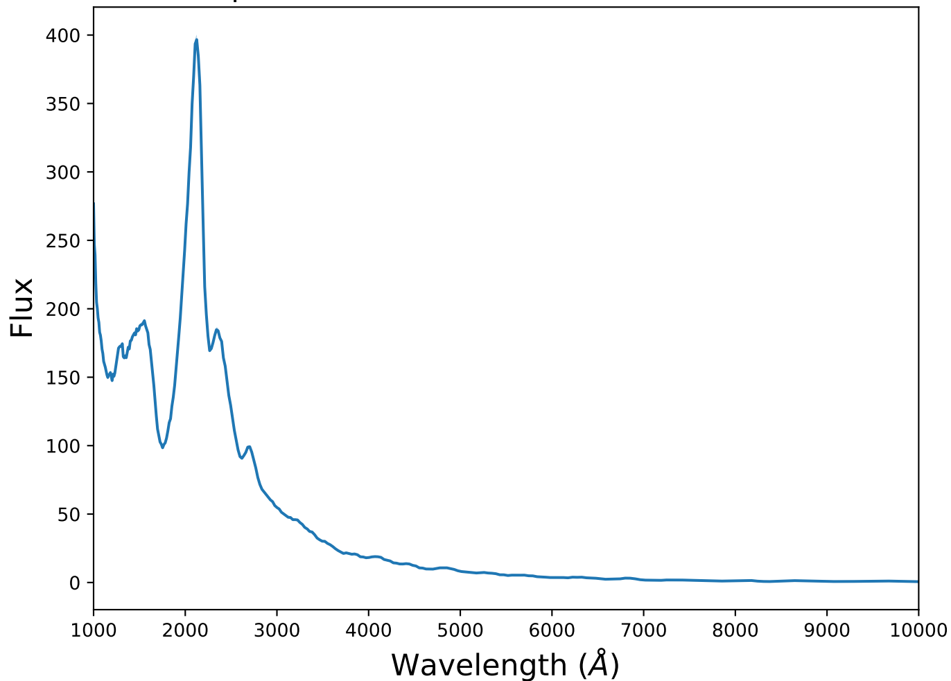
Spectrum 1 for transient TDE at z=1.27
